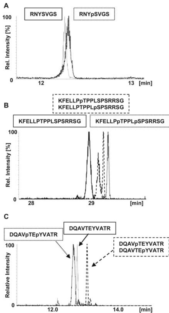
FIG. 1. Testing the elution order analyzing numerous peptides and their different phosphorylated cognates by LC/MS. A, normalized XICs of the peptide RNYSVGS ( unbroken line ) and its phosphorylated cognate RNYpSVGS ( dotted line ). B, normalized XICs of the peptide KFELLTPPLSPSRRSG ( unbroken line ), its singly phosphorylated cognates KFELLTPPLpSPSRRSG/KFELLpTPPLSPSRRSG ( broken line ), and its doubly phosphorylated complement KFELLpTPPLpSPSRRSG ( dotted line ). C, normalized XICs of the peptide DQAVTEYVATR ( unbroken line ), its singly phosphorylated cognates DQAVpTEYVATR/DQAVTEpYVATR ( broken line ), and its doubly phosphorylated complement DQAVpTEpYVATR ( dotted line ). Rel. , relative.
