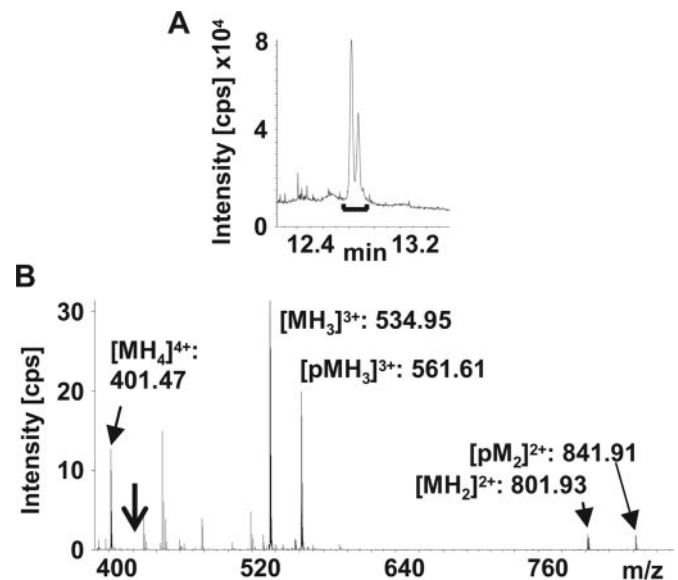
Fig. 4. LC/MS analysis of a 2:1 mixture of GLGTRTGSNLDK (M) and GLGTRTGPnLDK (PM). TIC (A) and the corresponding mass spectrum (B) summed from 12.74 to 12.94 min.
