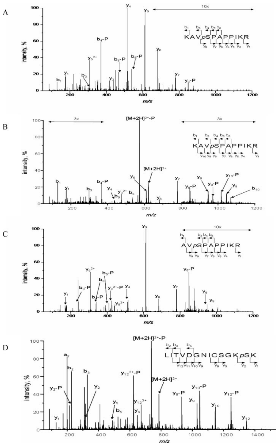
FIG. 2. CID tandem mass spectra of phosphopeptides detected after \text{TiO}_2 affinity enrichment. A, [\text{M} + 3\text{H}]^{3+} triply charged molecular ion at m/z 415.21 eluted between 20.5 and 21.0 min (Fig. 1B). B, [\text{M} + 2\text{H}]^{2+} , doubly charged molecular ions at m/z 622.32 eluted between 20.5 and 21.0 min (Fig. 1B). C, [\text{M} + 2\text{H}]^{2+} , doubly charged molecular ion at m/z 558.27 eluted between 21.6 and 22.1 min (Fig. 1C). D, [\text{M} + 2\text{H}]^{2+} , doubly charged molecular ion at m/z 786.34 of phosphopeptide eluted between 25.0 and 25.7 min (Fig. 1D). Neutral loss of phosphoric acid ( \text{H}_3\text{PO}_4 ) is indicated as “-P.”
