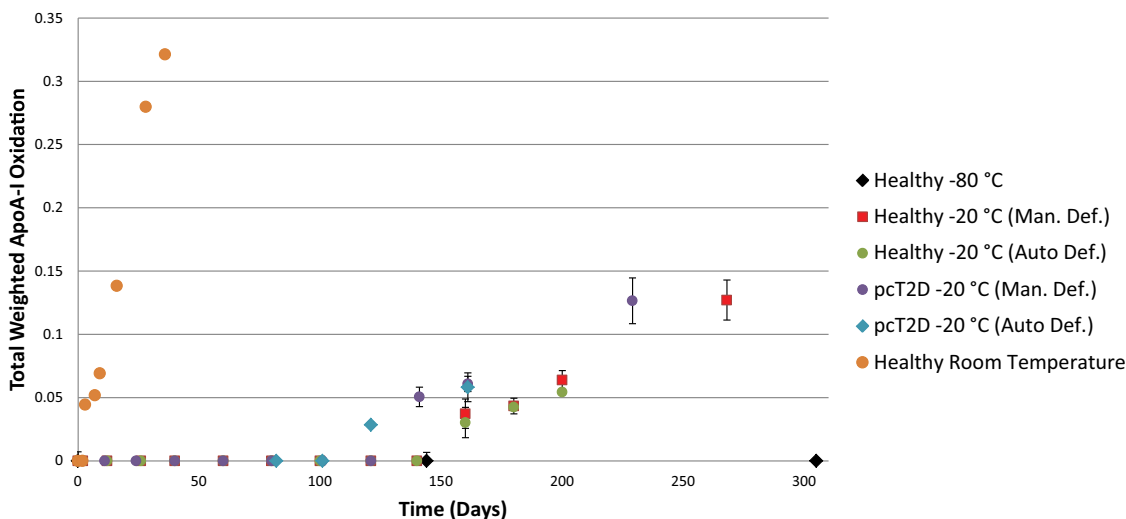
FIG. 3. Apolipoprotein A-I oxidation in plasma over time at -80\text{ }^{\circ}\text{C} , -20\text{ }^{\circ}\text{C} , and room temperature ( 25\text{ }^{\circ}\text{C} ). All samples were collected fresh and started on Day 0 with no oxidation. Up to three oxidation events may occur per apoA-I molecule, and total weighted oxidation was calculated as described in the text. Samples were the same as those described in Fig. 2.
