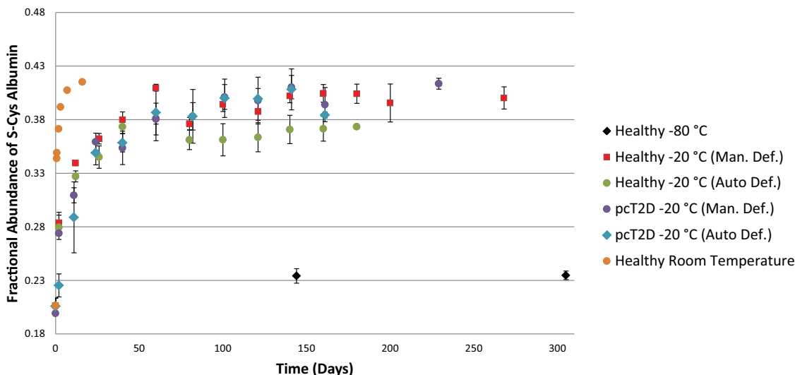
FIG. 2. Increasing abundance of S-cysteinyLATED albumin in plasma over time at -80\text{ }^{\circ}\text{C} , -20\text{ }^{\circ}\text{C} , and room temperature ( 25\text{ }^{\circ}\text{C} ). One sample was collected from a single healthy donor and a second sample was obtained from a single poorly controlled type 2 diabetic (pcT2D) with a history of coronary artery disease and myocardial infarction. Both samples were collected fresh and started on Day 0 at \sim 0.20 . Each sample was then aliquoted into two sets of three different vial types and stored in either an auto-defrost ( n = 3 ) or a manual-defrost freezer ( n = 3 ). An additional aliquot from the healthy donor was set aside for the room temperature time course. Auto-defrost freezers caused sublimation and/or evaporation of P/S water, resulting in sample dehydration (supplemental Fig. S7). Storage in such freezers is not recommended. Shown is the average \pm S.E. of three aliquots per point (fewer for later auto-defrost freezer points as a result of sublimation-mediated sample loss), stored (to no effect; supplemental Fig. S8) in different types of vials with different headspaces and degrees of sealing. If no error bars are shown, only one aliquot was analyzed. The slight initial increase in the sample stored at -80\text{ }^{\circ}\text{C} is likely due to the fact that the sample was measured and then aliquoted; during the aliquoting process the sample was at 4 - 25\text{ }^{\circ}\text{C} for over an hour. The first time point for the room temperature sample was measured at 17.5 h.
